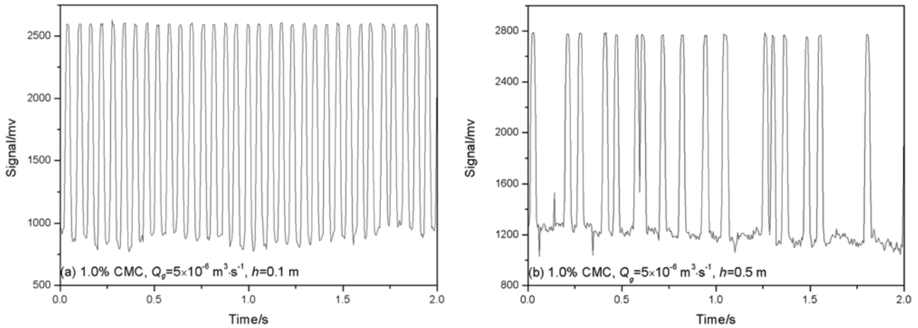
Fig. 4. Typical temporary signal of bubble passages in 1.0% CMC, Q_g = 5 \times 10^{-6} \text{ m}^3 \cdot \text{s}^{-1} , (a) h=0.1 m; (b) h=0.5 m.
